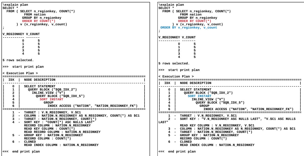
Figure 8 ORDERBY elimination
