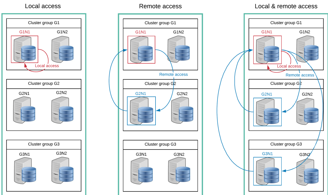
Figure 30 Cluster access
