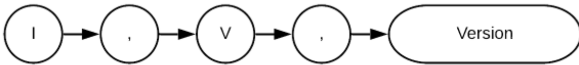
Figure 8 Version expression
