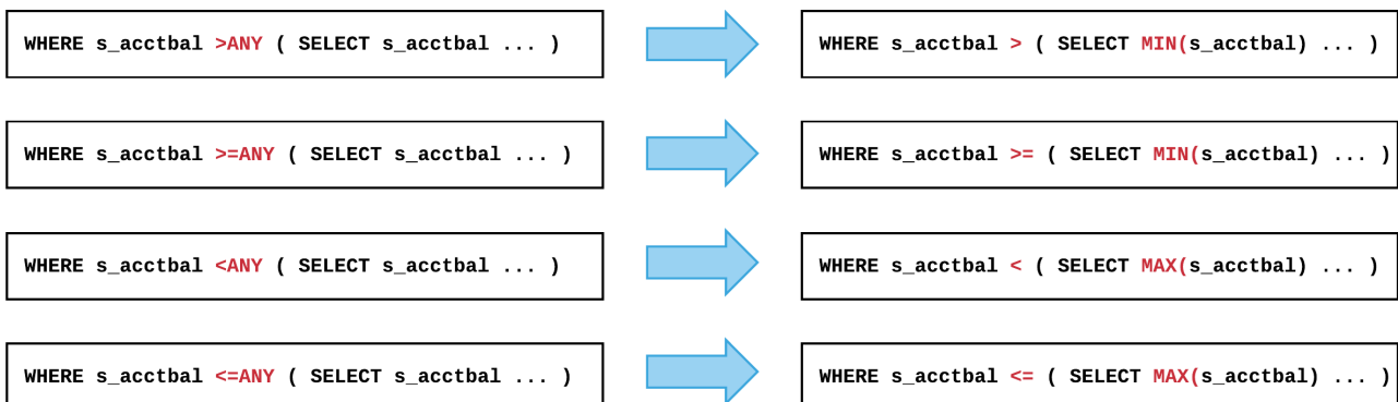
Figure 10 Quantifier elimination
