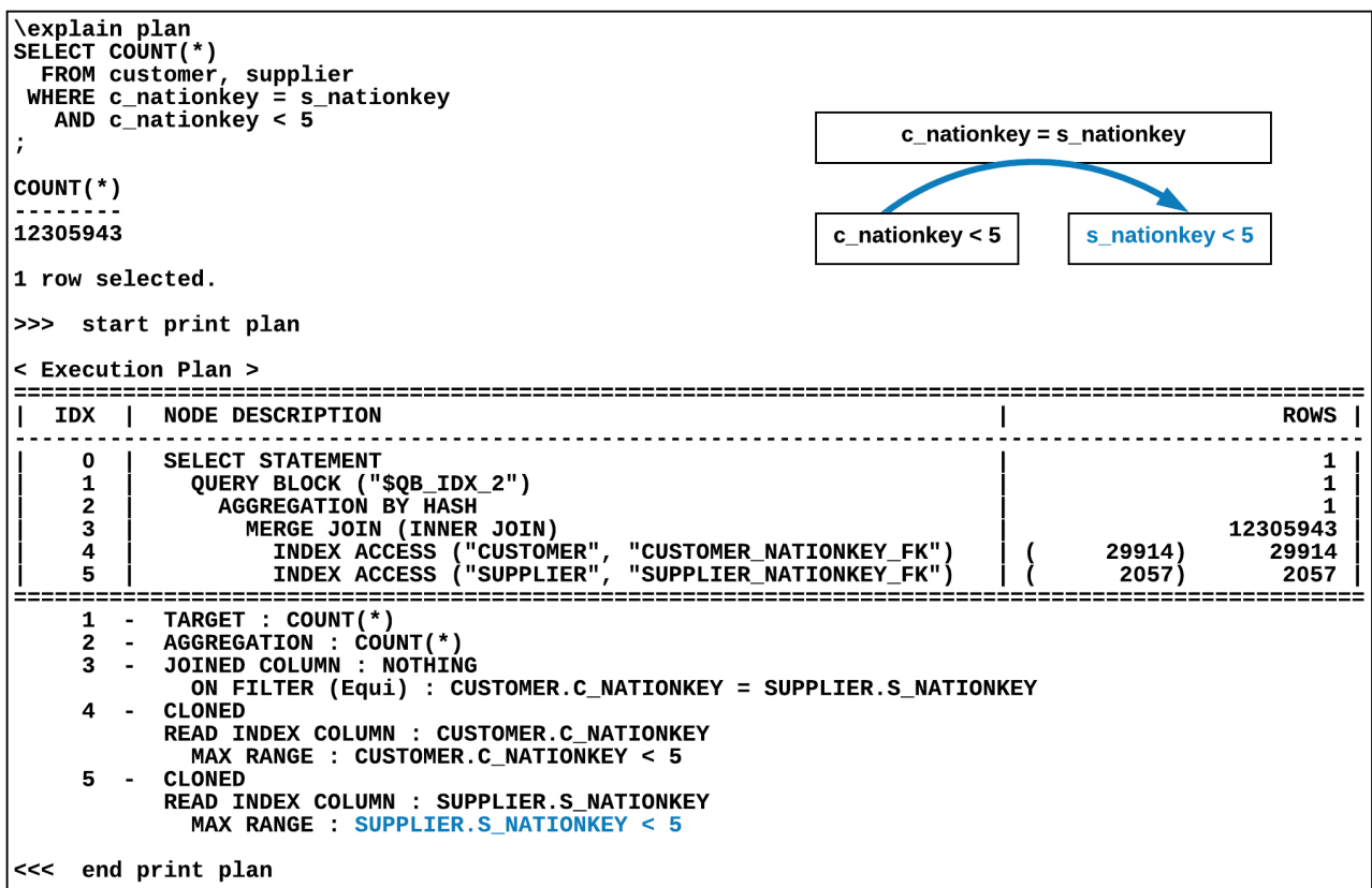
Figure 11 Transitive closure
