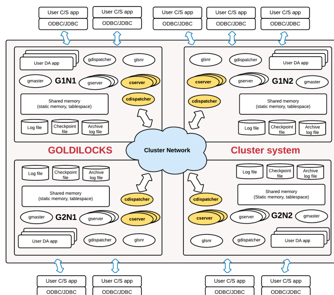
Figure 2 GOLDILOCKS cluster system architecture
